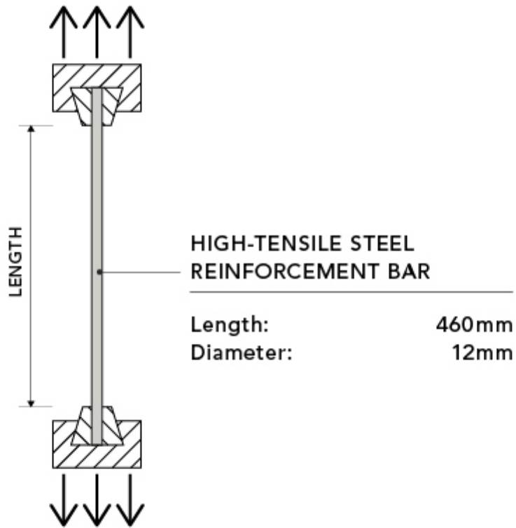
LOADING CONFIGURATION
