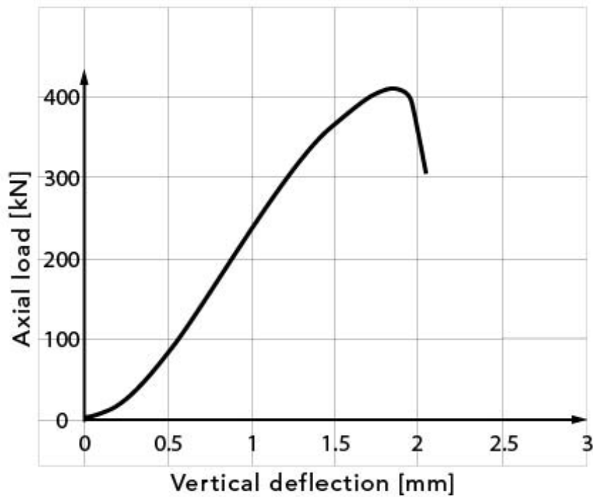
LOAD-DEFLECTION GRAPH
