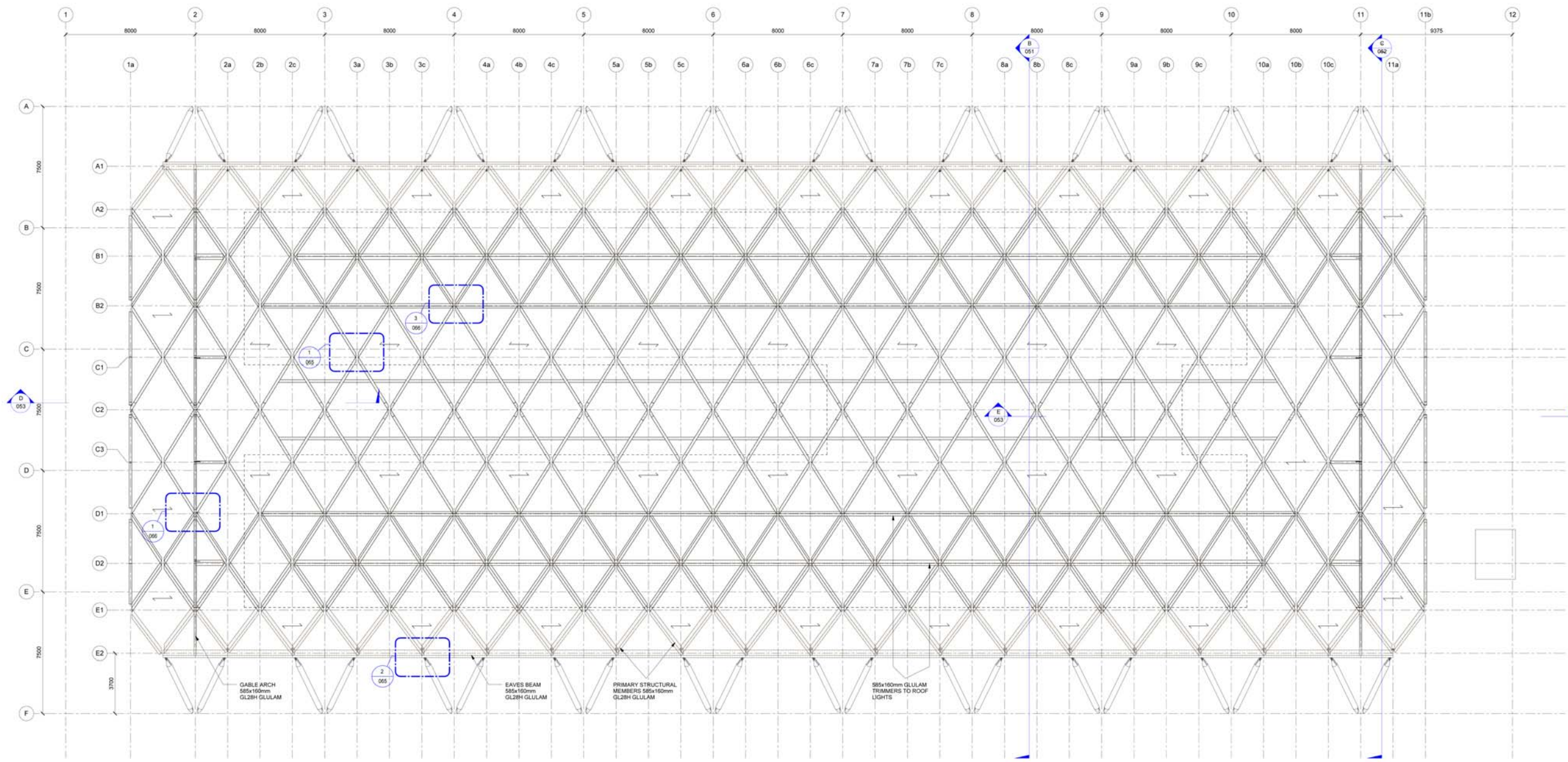
ROOF LAYOUT SCALE 1 : 100
